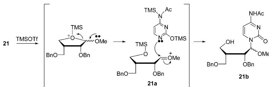
Scheme 4. Ring-opened product 21b formed during condensation of 21 with cytosine.
