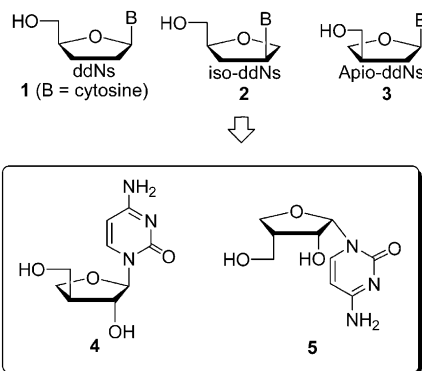
Figure 1. The rationale for the design of the target nucleosides.
