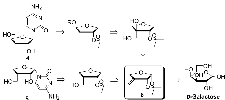
Scheme 1. Retrosynthetic analysis of the target nucleosides 4 and 5 .
