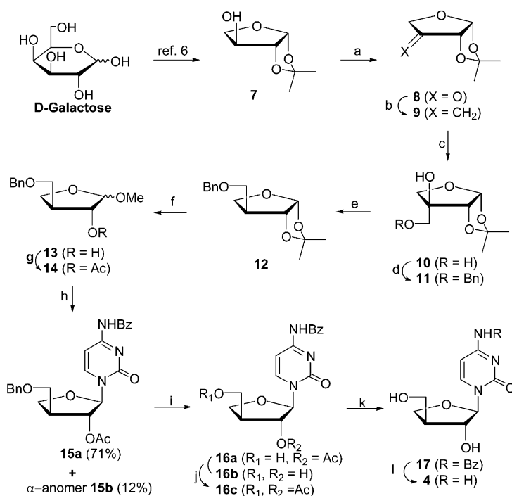
Scheme 2. Reagents: (a) PCC, 4A MS, CH 2 Cl 2 , rt, overnight, 68%; (b) CH 3 PPh 3 Br, NaH, t -amyl alcohol, THF, rt, 2 h, 80%; (c) OsO 4 , NMO, acetone: H 2 O (4:1), rt, 4 h, 98%; (d) n -Bu 3 SnO, toluene, 140 °C, 2 h and then, n -Bu 4 NBr, BnBr, 90–100 °C, overnight, 73%; (e) (i) NaH, THF, rt, 1 h and then, CS 2 , MeI, rt, 1 h; (ii) n -Bu 3 SnH, Et 3 B, benzene, rt, 3 h, 70% from 11 ; (f) p -TsOH, MeOH, rt, overnight, 75%; (g) Ac 2 O, DMAP, pyridine, rt, 1 h, 86%; (h) silylated N4-benzoylcytosine, TMSOTf, CH 3 CN, rt, overnight; (i) BCl 3 , CH 2 Cl 2 , –78 °C, 2 h; (j) Ac 2 O, pyridine, rt, overnight, 52% from 15a ; (k) K 2 CO 3 , MeOH, CH 2 Cl 2 , –5 °C, 40 min, 70%; (l) NaOMe, MeOH, rt, overnight, 92%.
