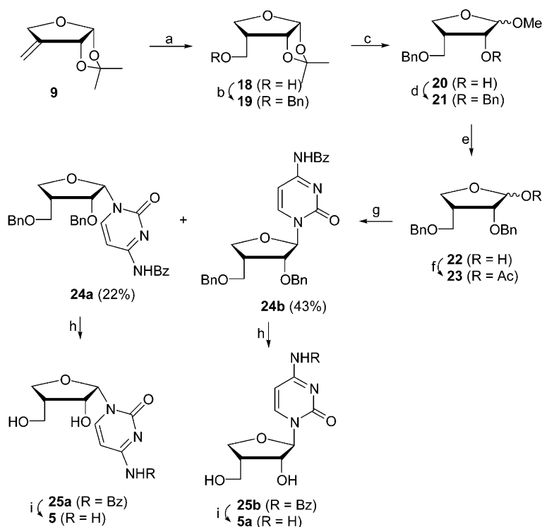
Scheme 3. Reagents: (a) 9-BBN, THF, 0 °C, 3 h and then, NaBO 3 , H 2 O, rt, overnight, 70%; (b) BnBr, NaH, n -Bu 4 NI, THF, rt, overnight, 90%; (c) p -TsOH, MeOH, rt, 2 d, 97%; (d) BnBr, NaH, n -Bu 4 NI, THF, rt, overnight, 98%; (e) 8 N HCl, H 2 O:1,4-dioxane (1:2), rt, 2 d, 95%; (f) Ac 2 O, pyridine, rt, overnight, 93%; (g) silylated N 4 -benzoylcytosine, TMSOTf, ClCH 2 CH 2 Cl, -35 °C, 1 h; (h) BCl 3 , CH 2 Cl 2 , -78 °C, 30 min, 68% for 25a , 70% for 25b ; (i) NaOMe, MeOH, rt, overnight, 97% for 5 , 81% for 5a .
